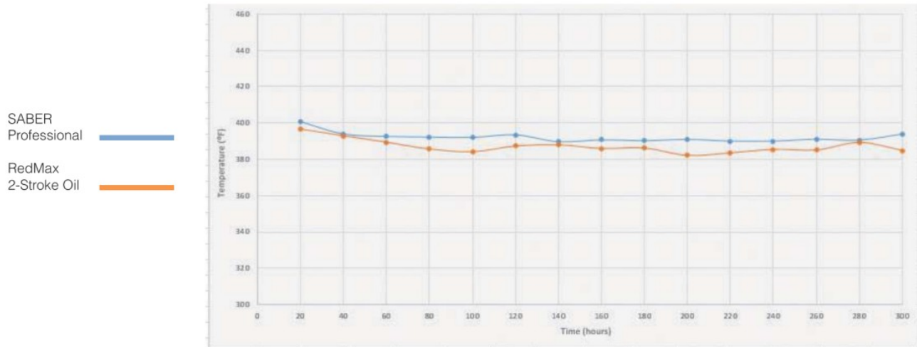
AVERAGE SPARK-PLUG TEMPERATURE @ WIDE-OPEN THROTTLE
