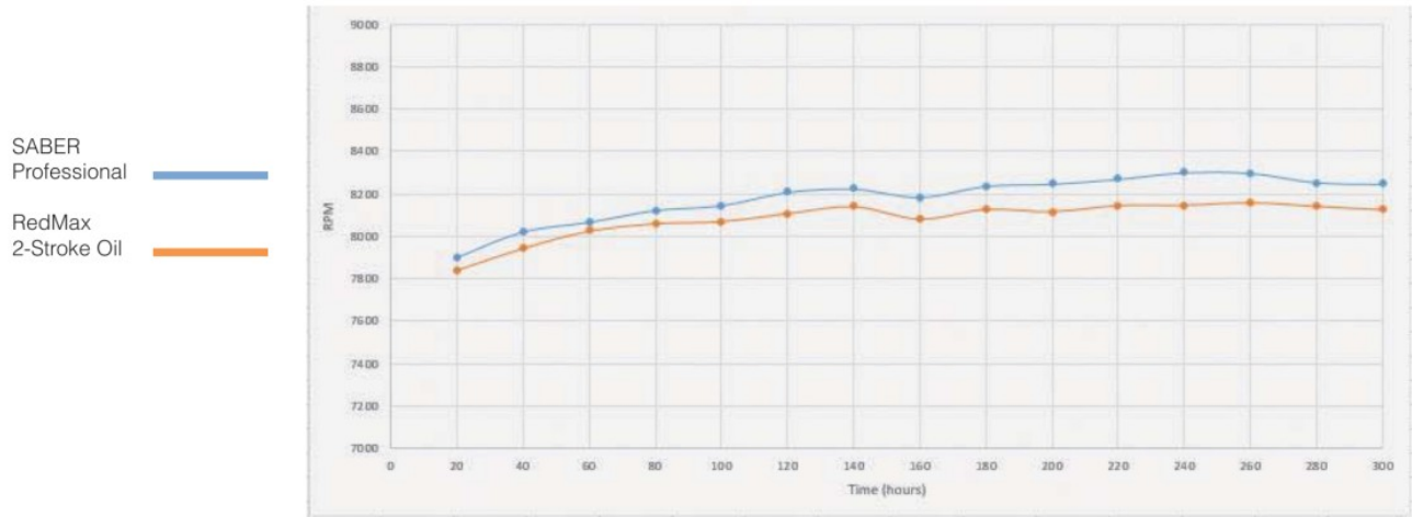
AVERAGE RPM @ WIDE-OPEN THROTTLE
